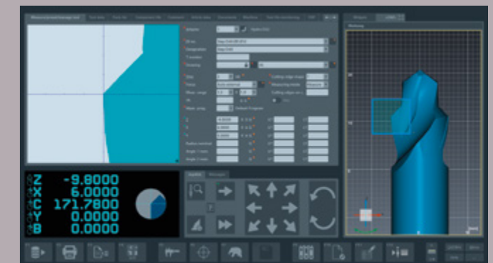
ZOLLER »caz« – the virtual measuring device for PC workstations for external creation of the inspection and measuring process including programs, nominal values and tolerances using the 3D model.
