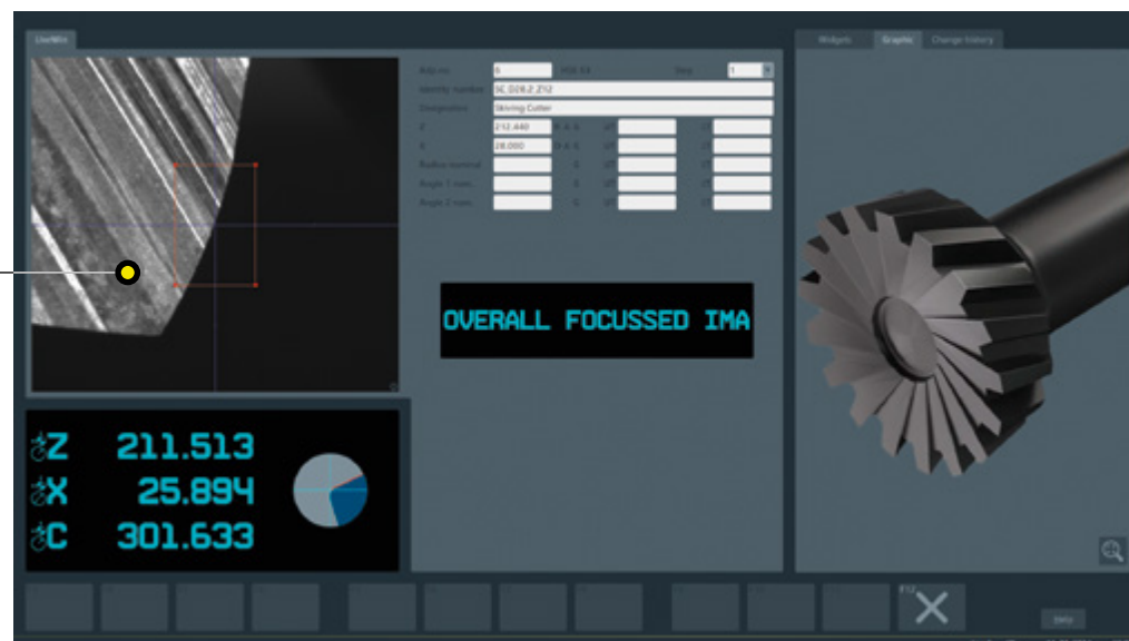
Power Skiving Cutter software – automatic measurement in incident light with the tool inspection camera, including depth image generation for distortion-free measurements and with automatic setting of the illumination intensity for optimal lighting of the surface.
