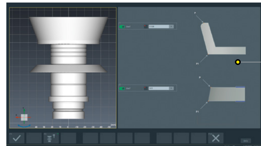
»elephant 2.0« for grinding wheels – scans the contour of the grinding wheel package and determines the individual grinding wheel types fully automatically. The package is then measured and recorded in detail without any data input. The grinding wheel pack can be saved for subsequent measurements.
