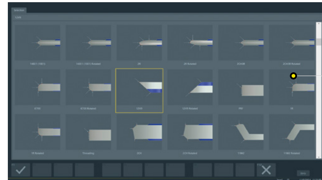
Grinding wheels software – library of grinding wheel types according to FEPA standard as well as grinding machine manufacturer specific types (e.g. ANCA, MAKINO, ROLLOMATIC).
