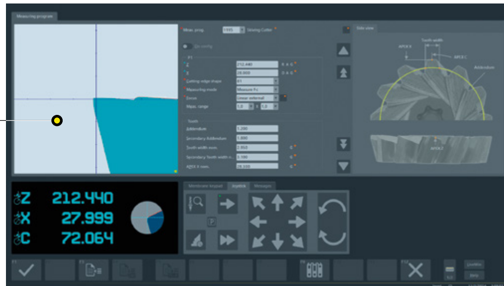
Power Skiving Cutter software – for determining the tool parameters required for use on the machine tool – photo-realistic input dialog and automatic measurement in incident and transmitted light.
