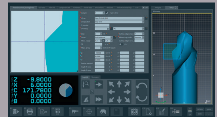
ZOLLER »caz« – the virtual measuring device for PC workstations for external creation of the inspection and measuring process including programs, nominal values and tolerances using the 3D model.
